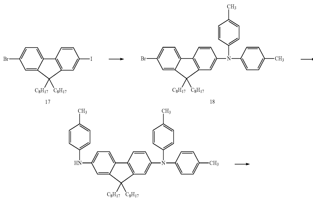
Reaction Scheme F
