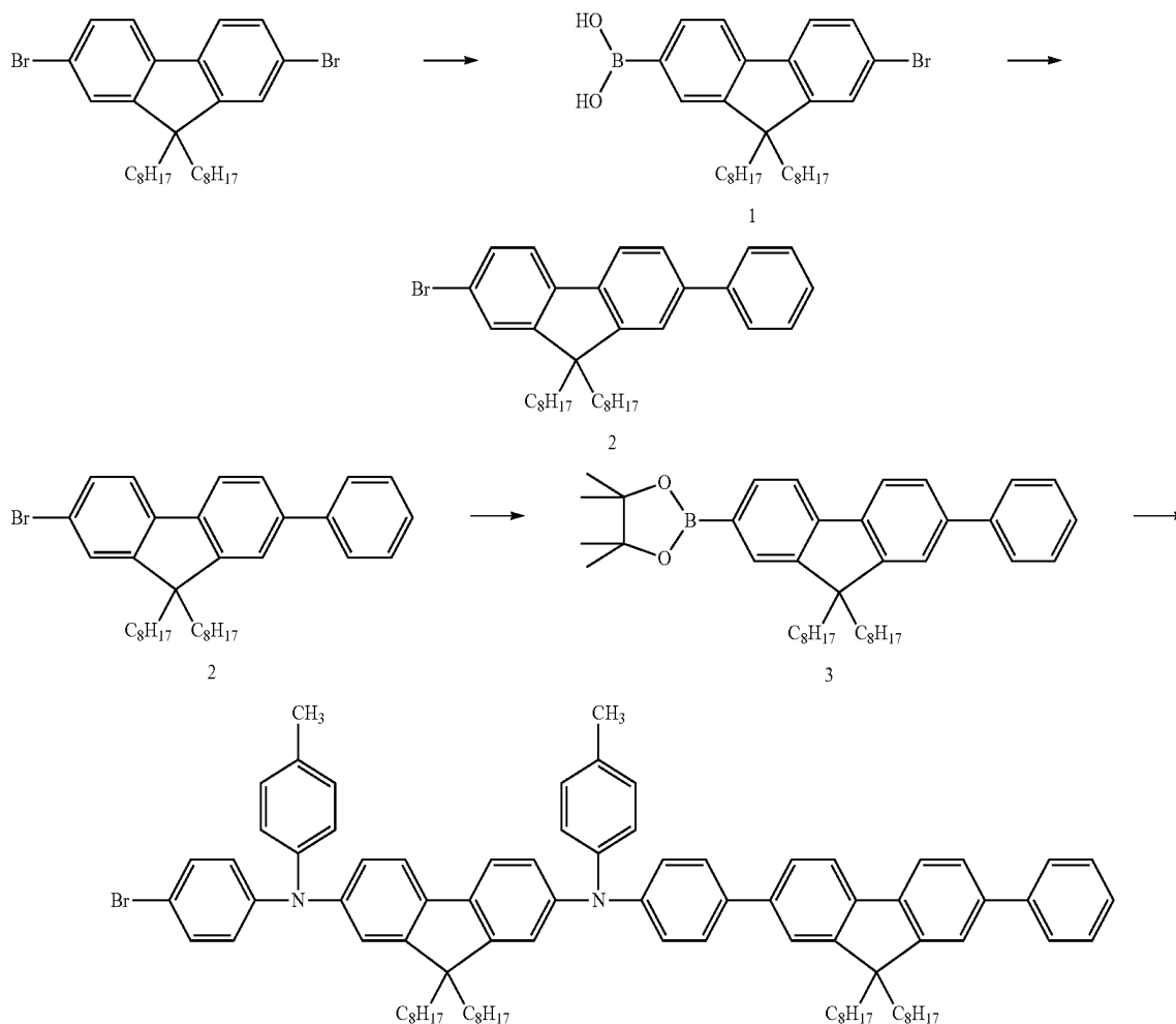
Reaction Scheme A
