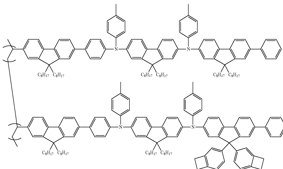
Compound 100
