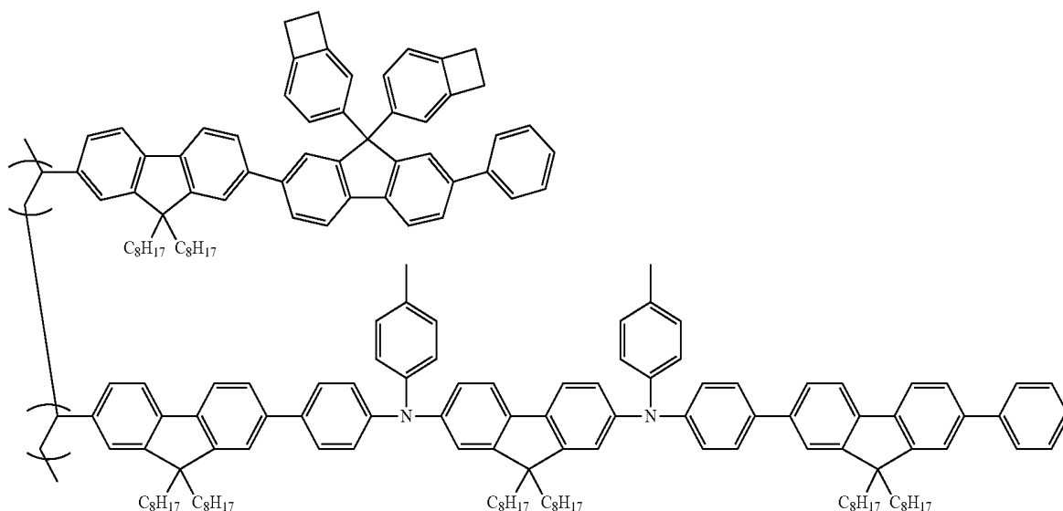
Compound 101
