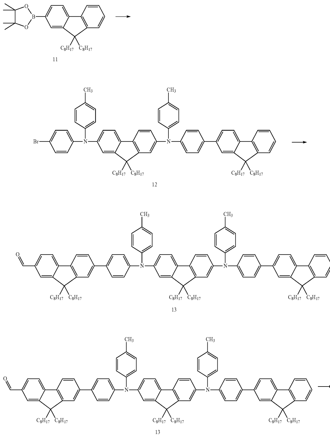
Reaction Scheme D
