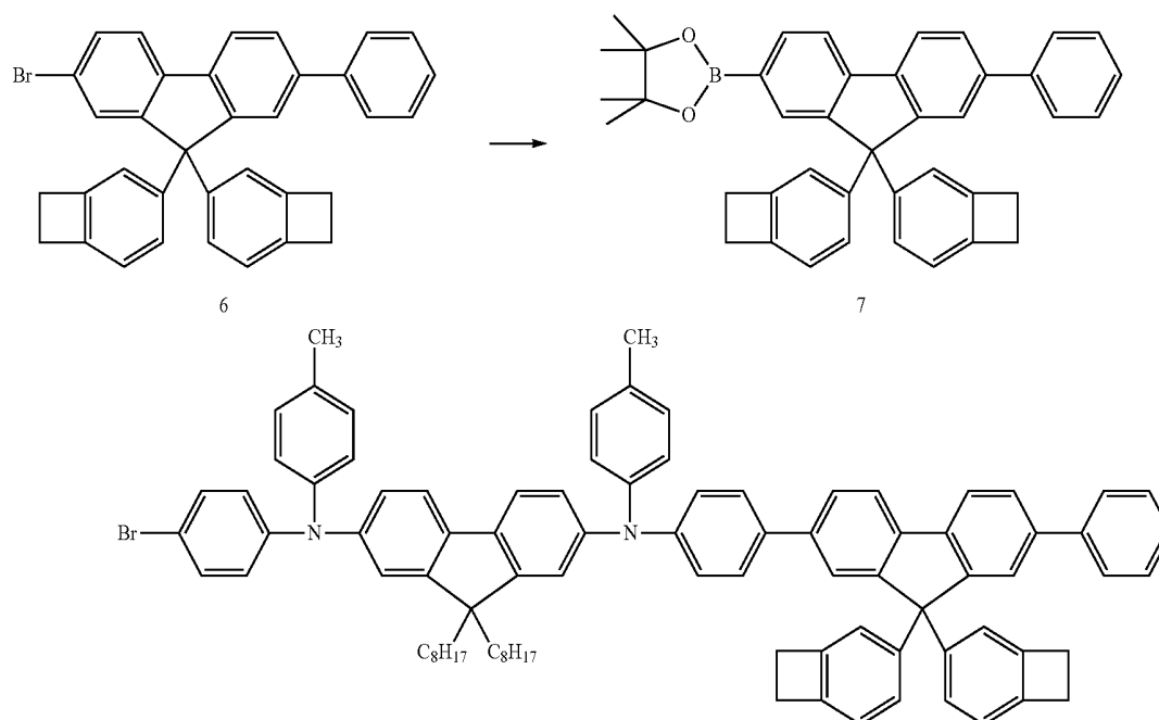
Reaction Scheme B
